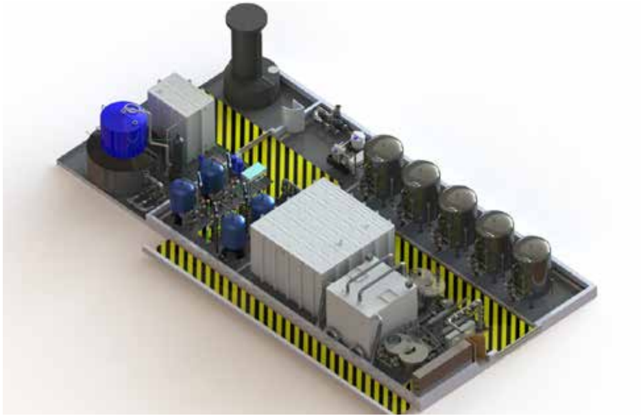
3D model of the incoming water treatment plant for Britvic.
